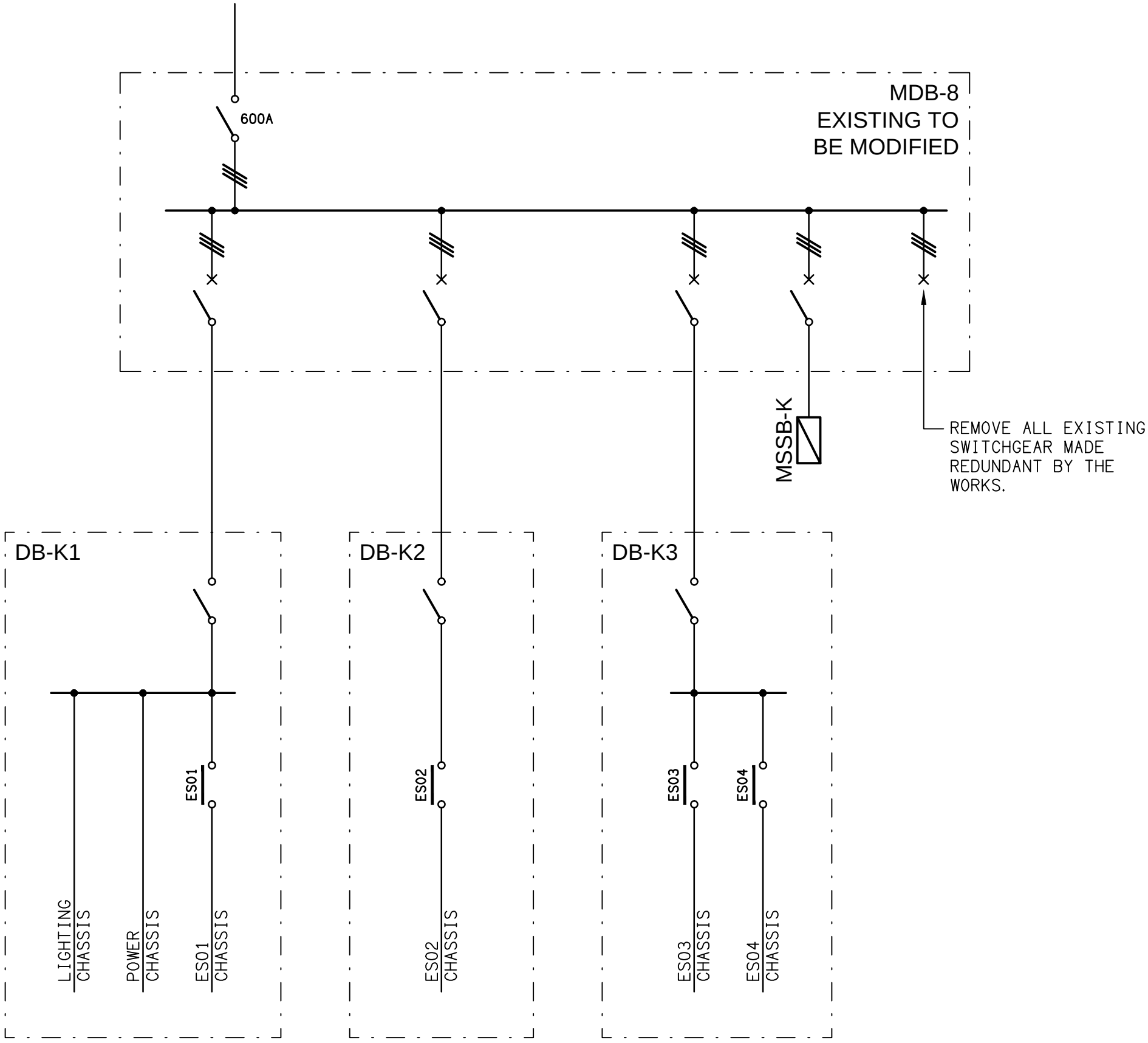
PROPOSED MDB-9 POWER SCHEMATIC NOT TO SCALE
